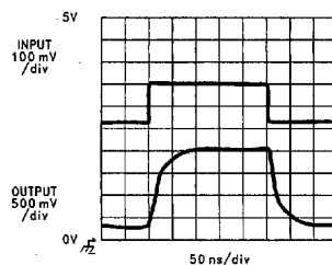
LM7131 Cable Driver A_V = +10 @ +3V
