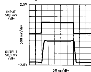
LM7131 Cable Driver A_V = +2 @ +3\text{V}
