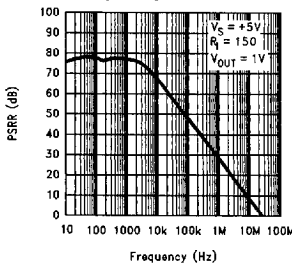
LM7131 PSRR vs Frequency @ 5V
