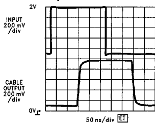
LM7131 Driving 75' RG-59 A_V = +2 @ +5V
