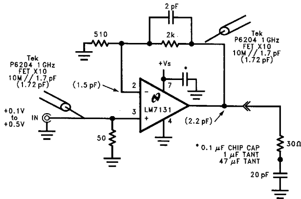
FIGURE 10. Flash A/D A_V = +5 with Feedback Capacitor
