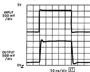
LM7131 Cable Driver A_V = +1 @ +5V
