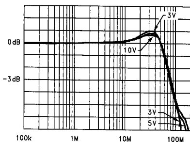
LM7131 Single Supply Bode Plot @ 3V, 5V and 10V
