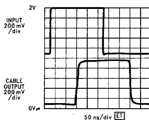
LM7131 Driving 75' RG-59 A_V = +2 @ +3V
