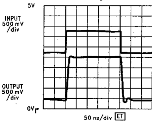
LM7131 Driving Flash A/D Load A_V = +2 @ +5V
