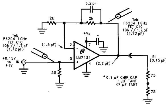
FIGURE 2. Cable Driver A_V = +2
