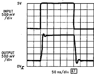
LM7131 Driving Flash A/D Load A_V = +1 @ +5V
