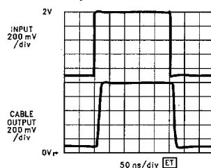
LM7131 Driving 5' RG-59 A_V = +2 @ +5V
