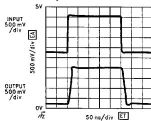
LM7131 Cable Driver A_V = +1 @ +3\text{V}
