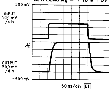
LM7131 Driving Flash A/D Load A_V = +10 @ +5V
