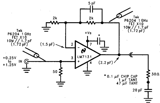
FIGURE 8. Flash A/D A_V = +2
