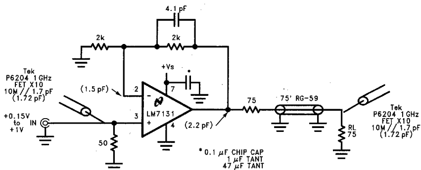
FIGURE 4. Cable Driver 75' RG-59
