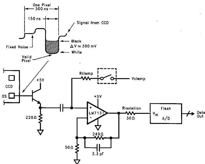
FIGURE 15. CCD Amplifier
