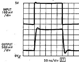
LM7131 Driving Flash A/D Load A_V = +5 @ +5V
