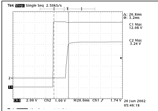
Figure 37. APC08F08 T ON delay at V IN,max = 12V.
