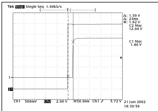
Figure 39. APC08Y08 T ON delay at V IN,max = 12V (Ch1)
