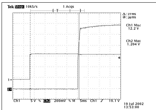
Figure 41. APC08K08 T ON delay at V IN,max = 12V.
