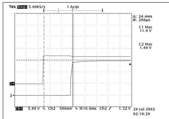
Figure 40. APC08M08 T ON delay at V IN,max = 12V.
