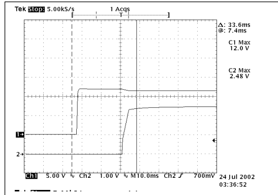
Figure 38. APC08G08 T ON delay at V IN,max = 12V.
