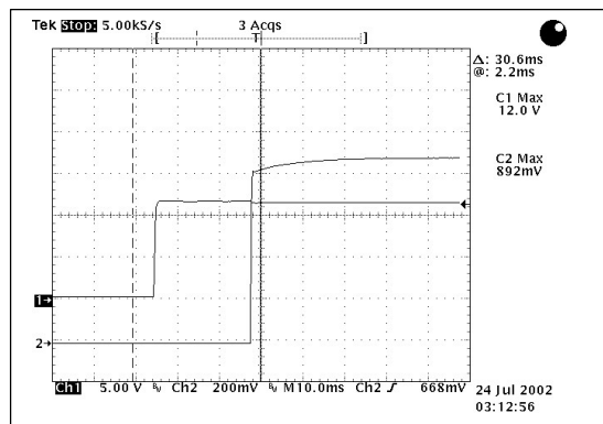
Figure 42. APC08J08 T ON delay at V IN,max = 12V.
