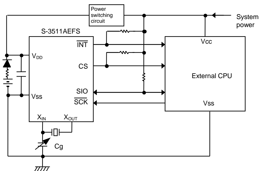
Figure 15 Applied circuit 1
