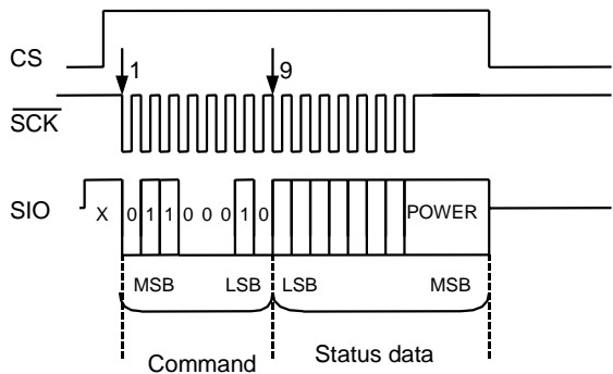
Figure 4 Write communication
