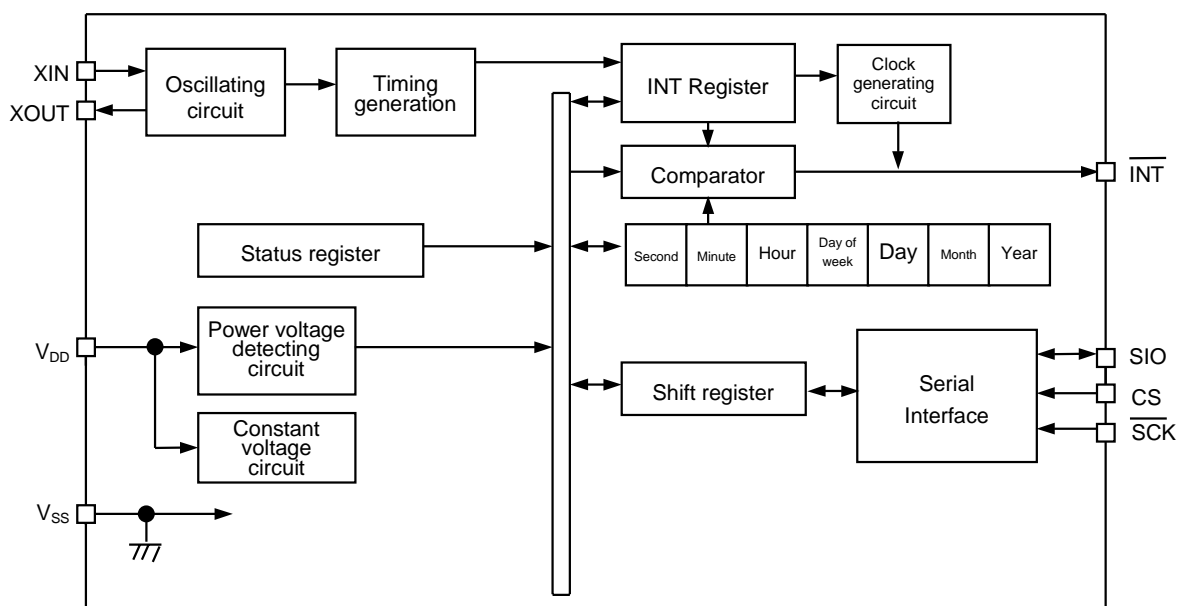
Figure 1 Block diagram
