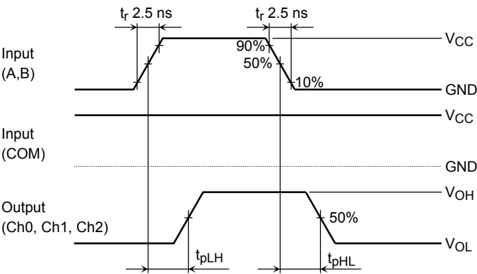
Figure 2 t_{pLH} , t_{pHL}
