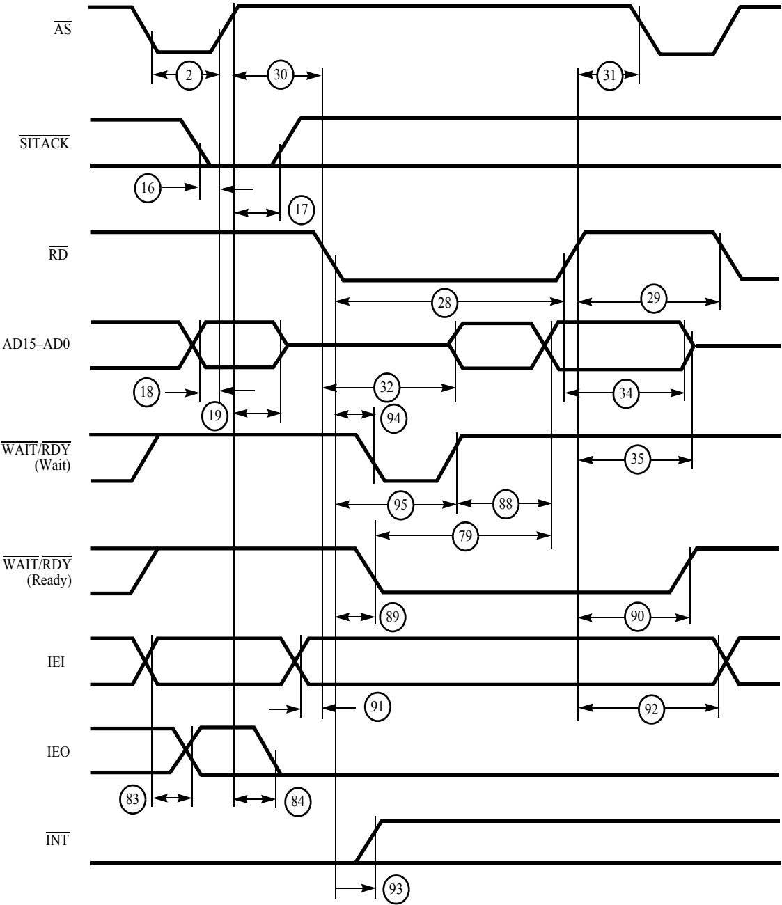
Figure 19. Multiplexed RD Interrupt Acknowledge Cycle
