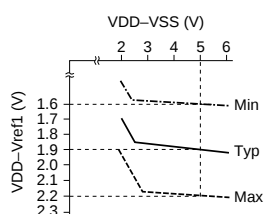
Figure 21 Voltage Characteristics between VDD and Vref1
