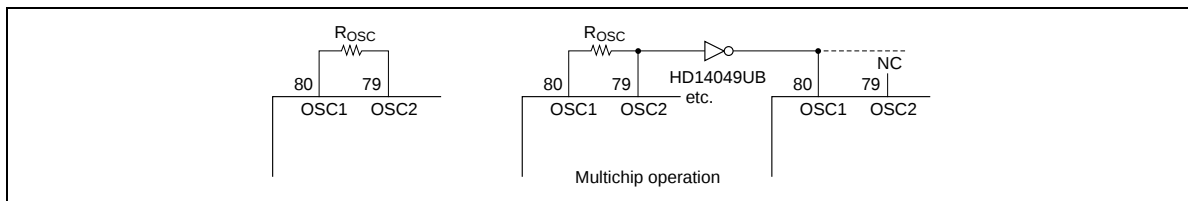
Figure 24 Example of Oscillation Circuit
