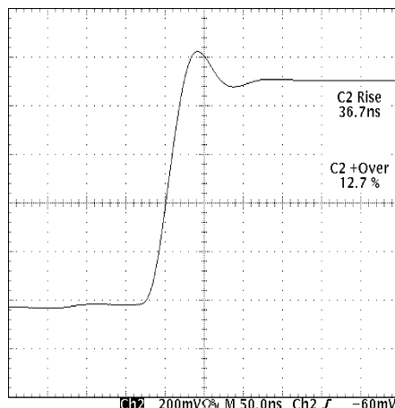
Figure 64. Rise Time
