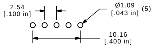
P.C. MOUNTING
