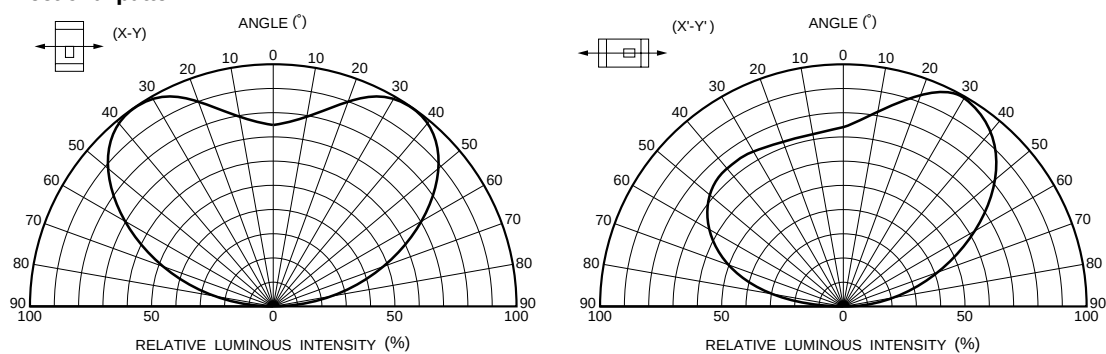
Fig. 1 Directional pattern
