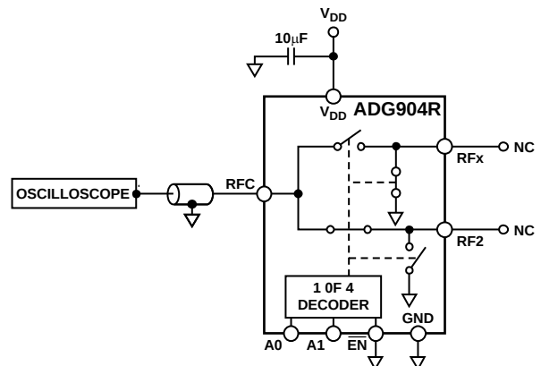
Figure 24. Video Feedthrough
