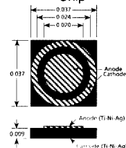
Figure 2 Chip
