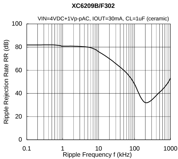
(10) Ripple Rejection Rate
