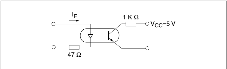
Figure 2. Switching operation (with saturation)
