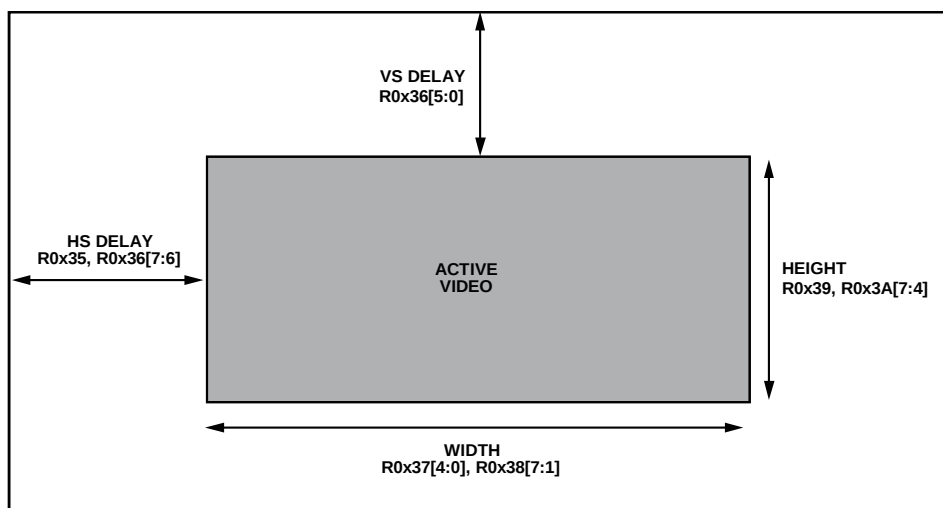
Figure 4. Active Video
