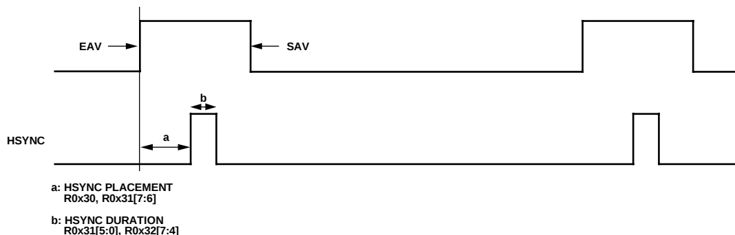
Figure 5. HSYNC Reconstruction
