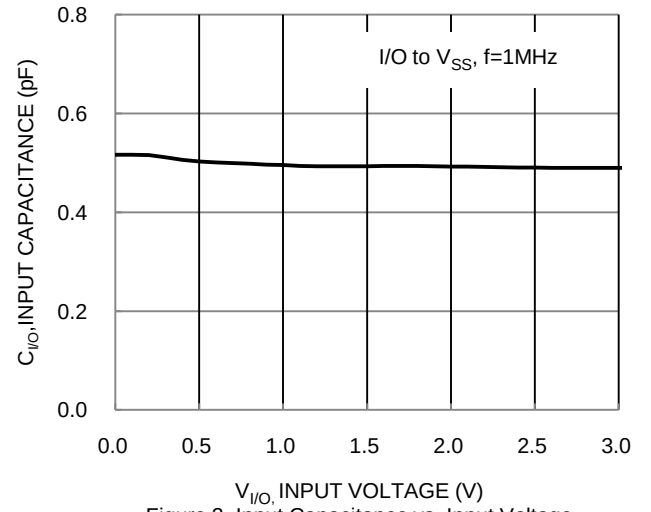
Figure 2. Input Capacitance vs. Input Voltage
