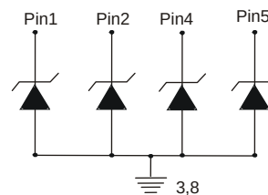
Device Schematic
