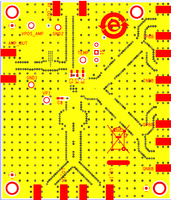
Figure 45. Layout of ADL5385-DIFFLO-EBZ, Bottom View
