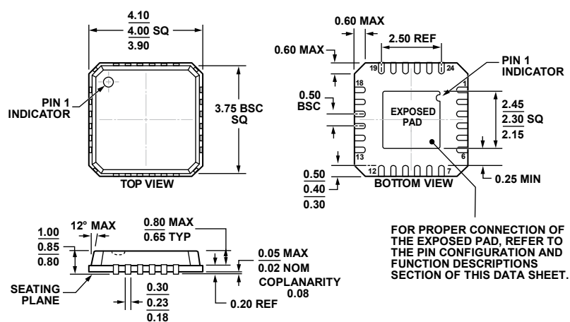
Figure 49. 24-Lead Lead Frame Chip Scale Package [LFCSP_VQ] 4 mm × 4 mm Body, Very Thin Quad (CP-24-2) Dimensions shown in millimeters
