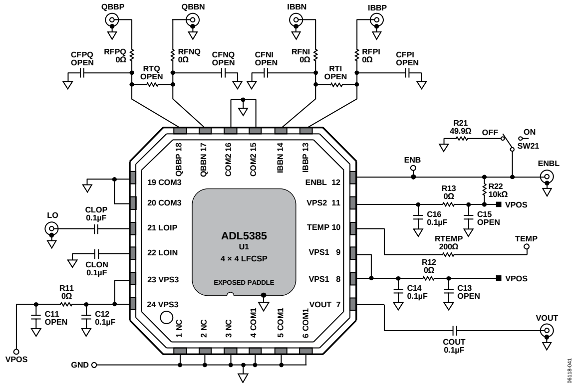
Figure 46. ADL5385-EVALZ Schematic
