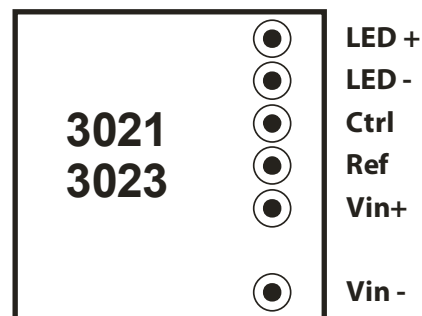
Figure 1. Bottom view Pinout of the 3021/3023 BuckPuck
