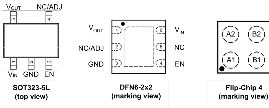
Figure 3. Pin configuration
