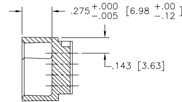
SECTION X-X
