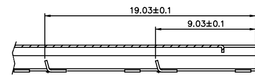
SEC. E-E (SCALE 3:1)
