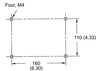
Mounting Holes
