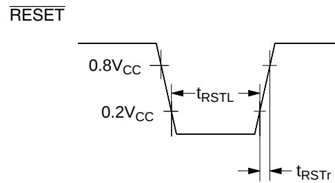
Figure 58 RESET Timing
