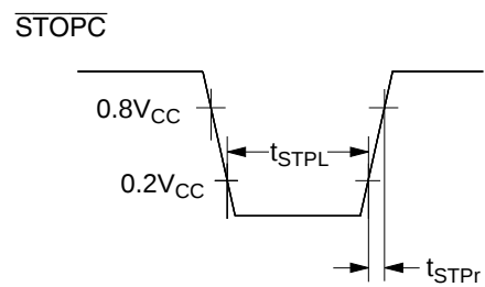
Figure 59 STOPC Timing
