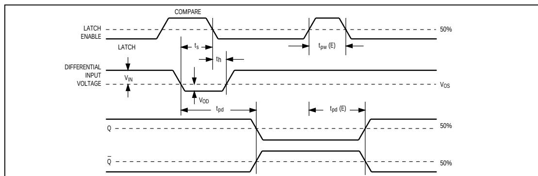
Figure 3. Timing Diagram
