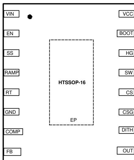
Figure 5-1. LM25088-1 16-Pin PWP Package (Dither Version) (Top View)
