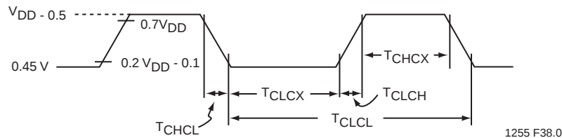
FIGURE 14-6: EXTERNAL CLOCK DRIVE WAVEFORM
