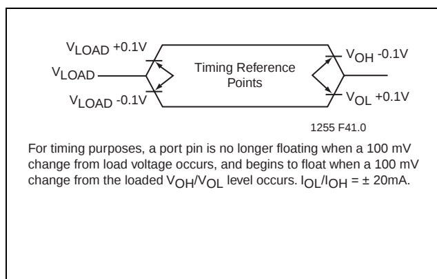
FIGURE 14-9: FLOAT WAVEFORM
