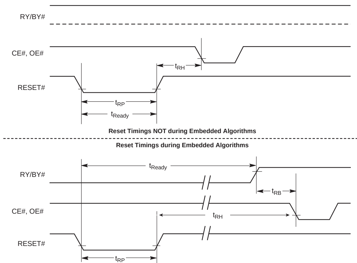
Figure 15.4 Reset Timings
