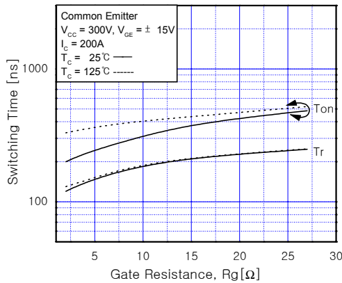
Fig 5. Turn-On Characteristics vs. Gate Resistance
