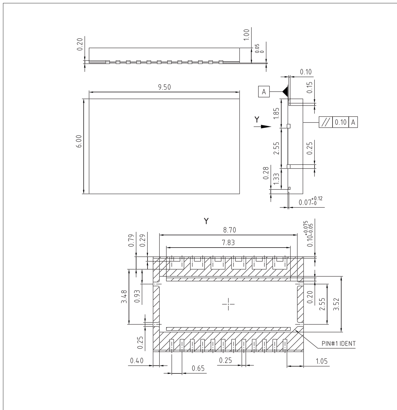
Figure 37 TSON-24-7 Package drawing
