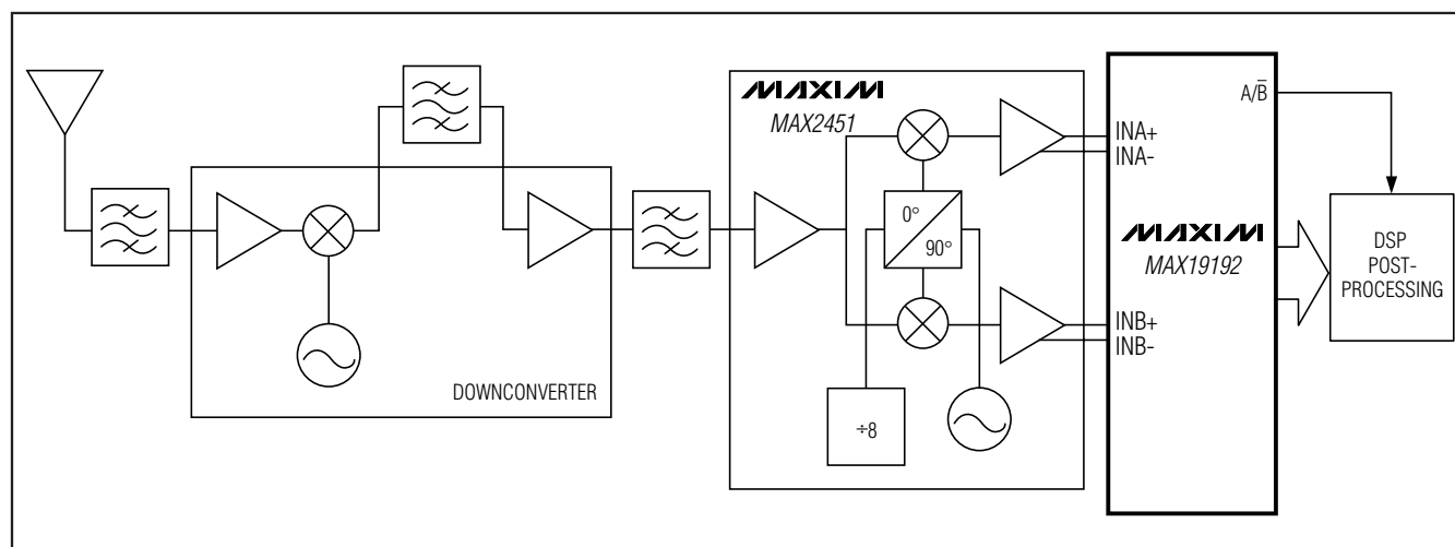
Figure 12. Typical QAM Receiver Application
