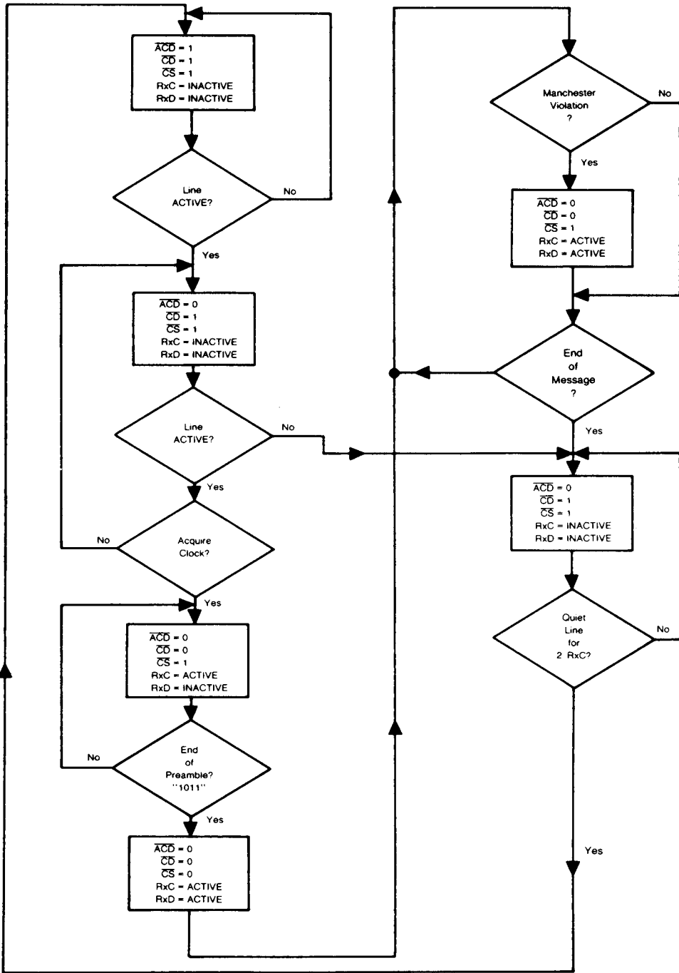
Figure 8. Am7960 Receive Flow Chart—Mode 0
