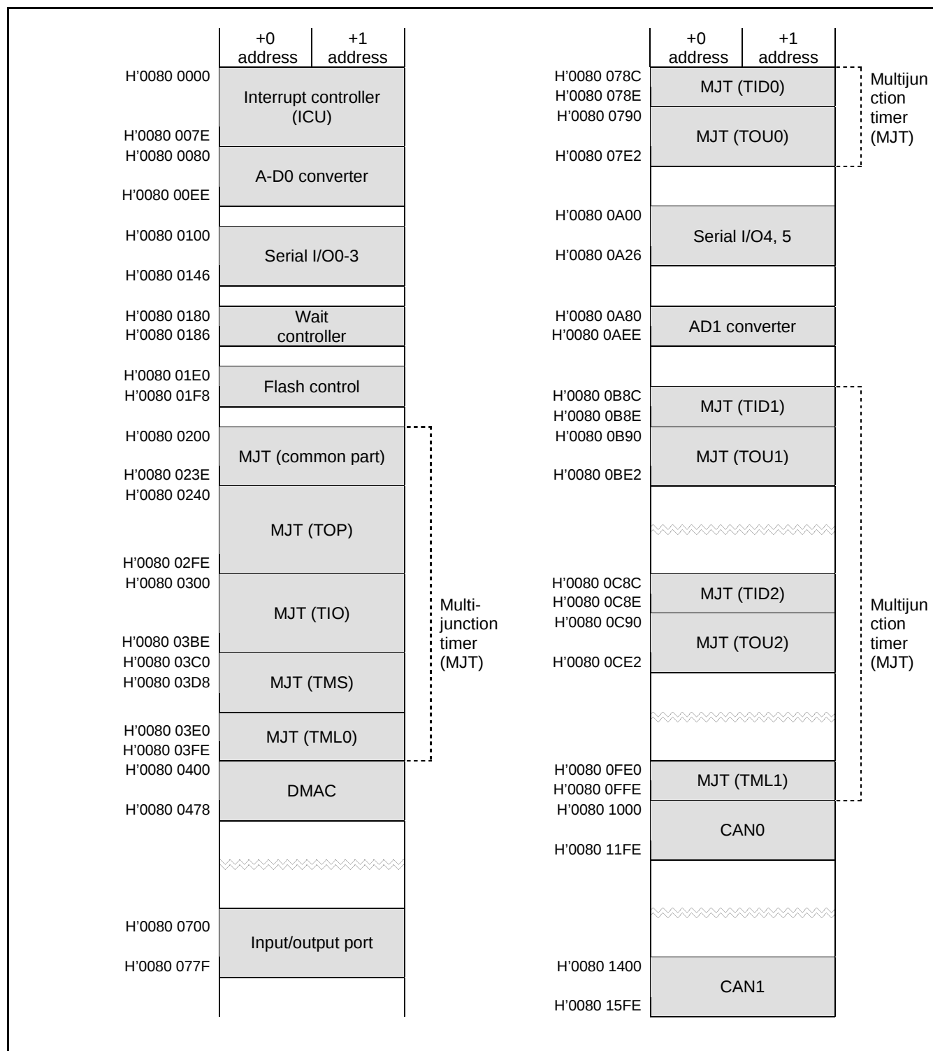
Figure 5. SFR Area
