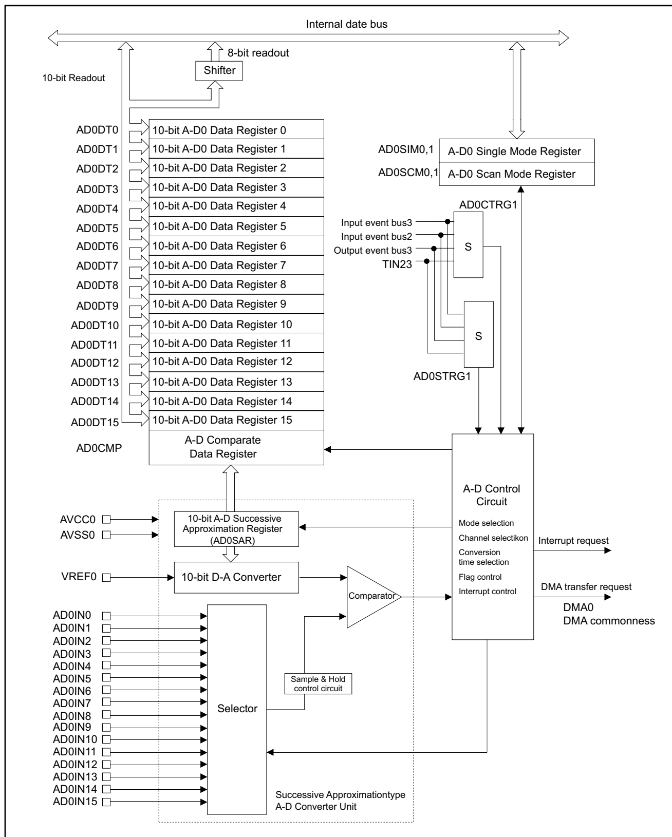
Figure 12. Block Diagram of the A-D0 Converter
