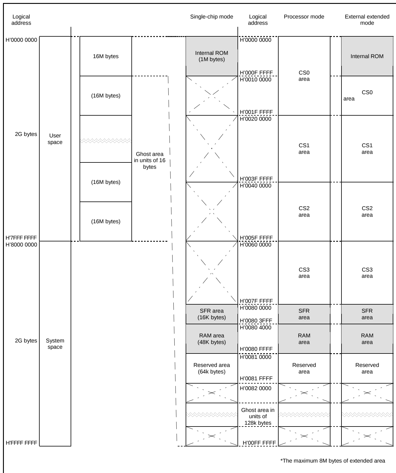
Figure 4. Address space
