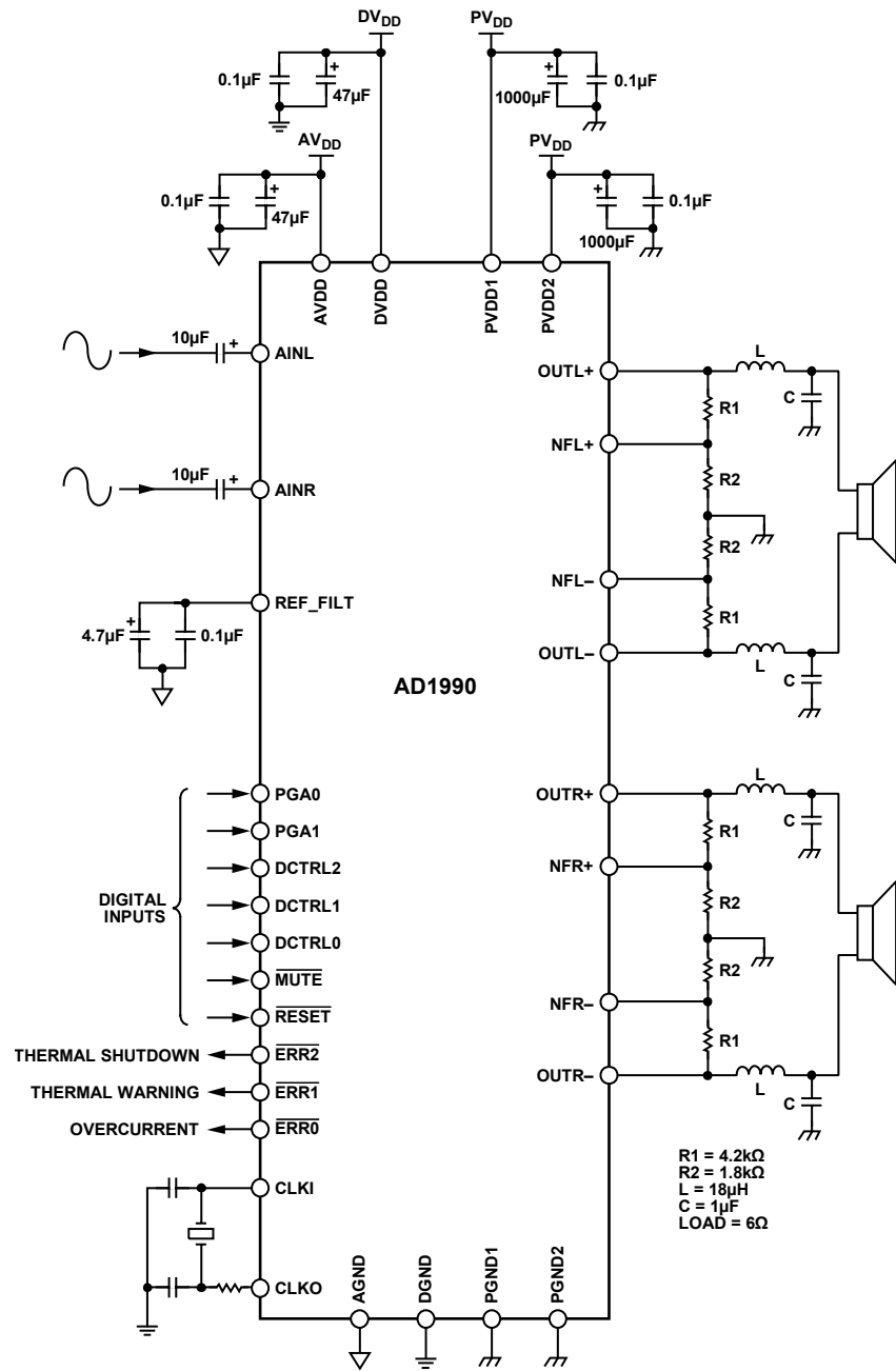
Figure 26. Typical Application Circuit
