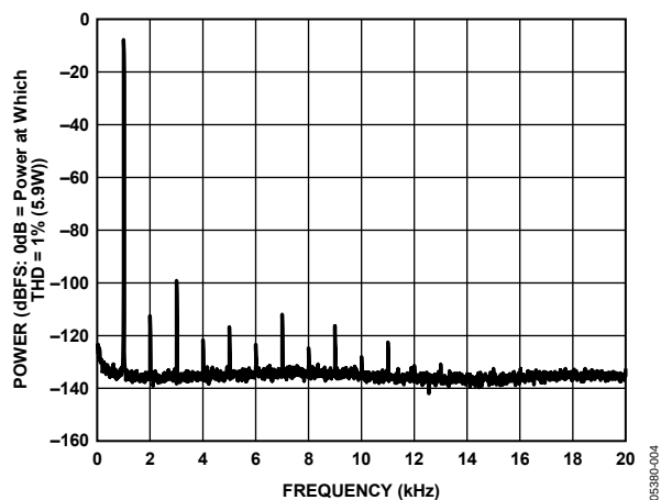
Figure 4. 1 W Output Power into 4 Ω Load
