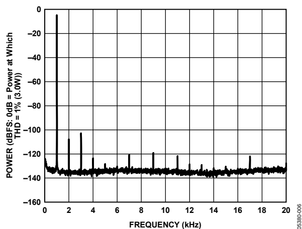
Figure 6. 1 W Output Power into 8 Ω Load
