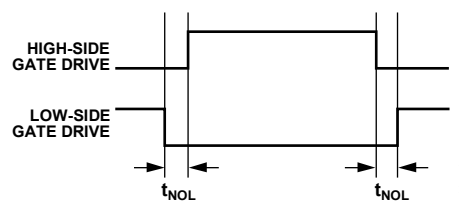
Figure 24. Half-Bridge Nonoverlap Delay Timing
