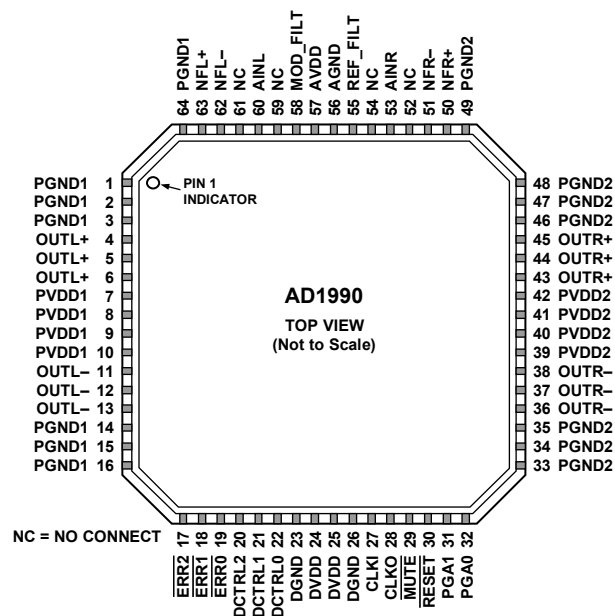
Figure 3. Pin Configuration
