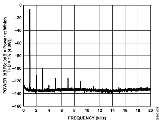
Figure 5. 1 W Output Power into 6 Ω Load
