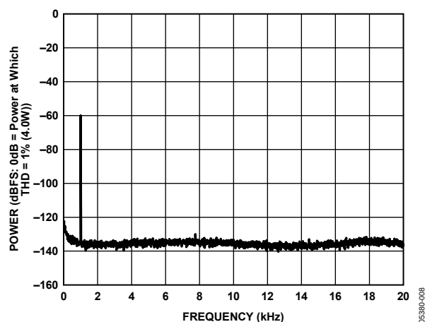
Figure 8. -60 dBFS Output Power into 6 Ω Load
