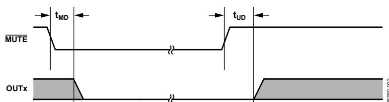
Figure 2. Mute and Unmute Delay Timing
