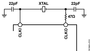
Figure 25. Crystal Connection
