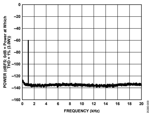
Figure 9. -60 dBFS Output Power into 8 Ω Load
