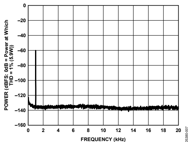
Figure 7. -60 dBFS Output Power into 4 Ω Load
