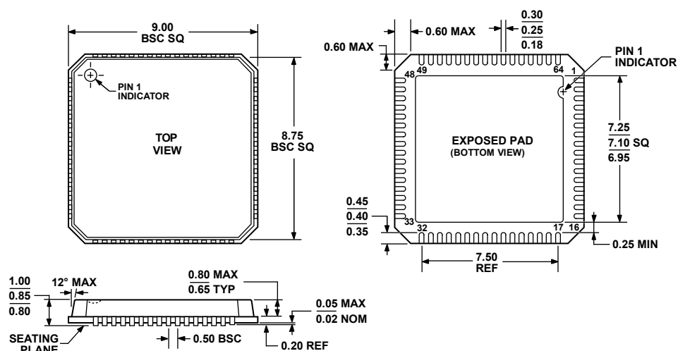
Figure 27. 64-Lead Lead Frame Chip Scale Package [LFCSP_VQ] 9 mm × 9 mm Body, Very Thin Quad (CP-64-3) Dimensions shown in millimeters
