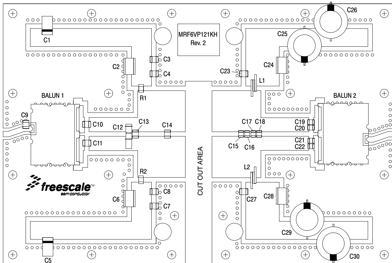
Figure 14. MRF6VP121K6(HSR6) Test Circuit Component Layout — 785 MHz
