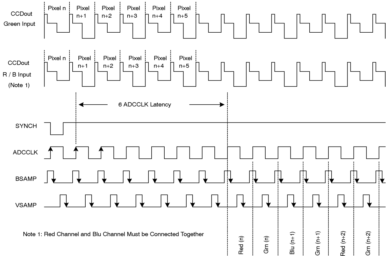
Graph 13. Two Channel G / RB Mode Synchronization and ADC Timing
