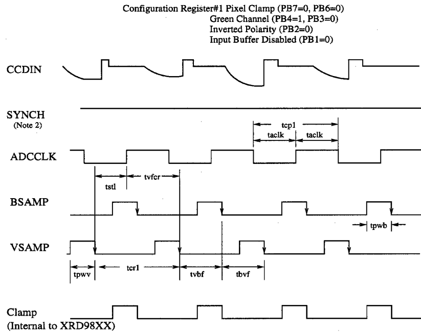
Graph 3. 1 Channel CDS Mode – Pixel Clamp
