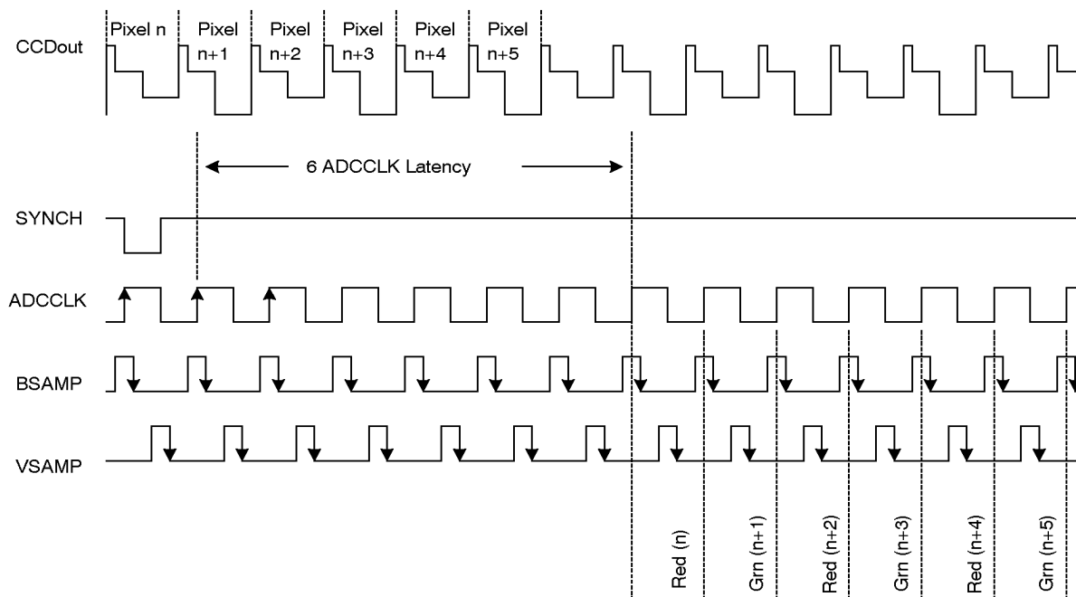
Graph 12. (A) Single Channel Bayer Mode Synchronization and ADC Timing
