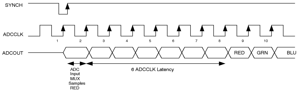
Graph 14. XRD9812 Timing For SYNCH/ADCCLK/ADCOUT
