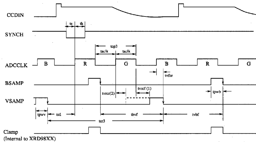
Graph 1. 3 Channel CDS Mode – Pixel Clamp
