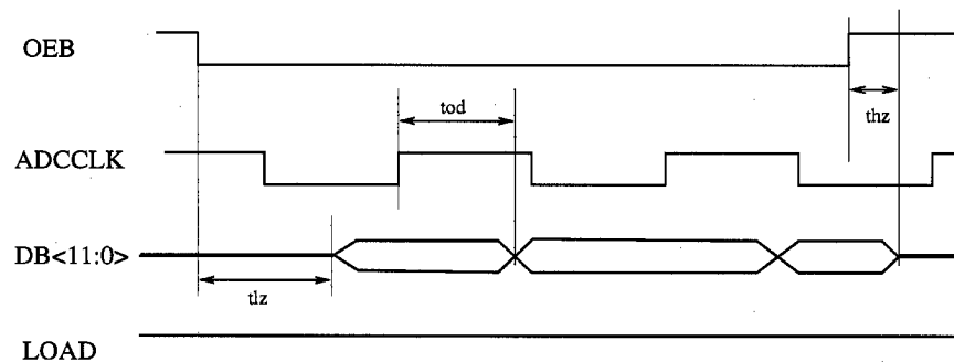
Graph 11. ADC Digital Output Timing
