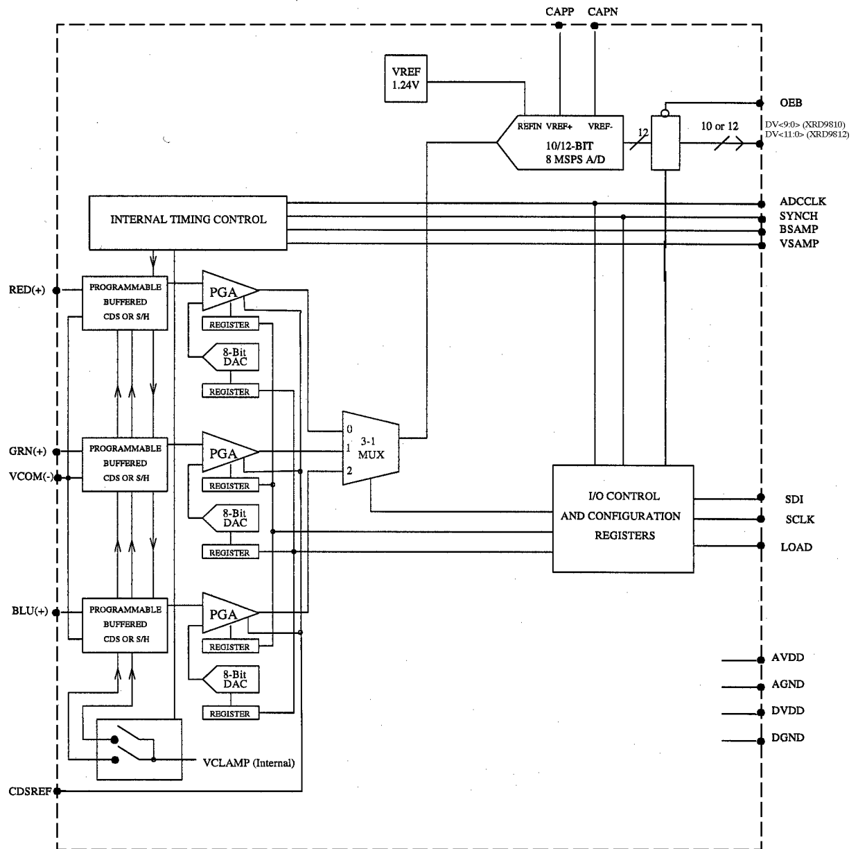
Figure 1. XRD9810/12 Functional Block Diagram (32 Pin Count)
