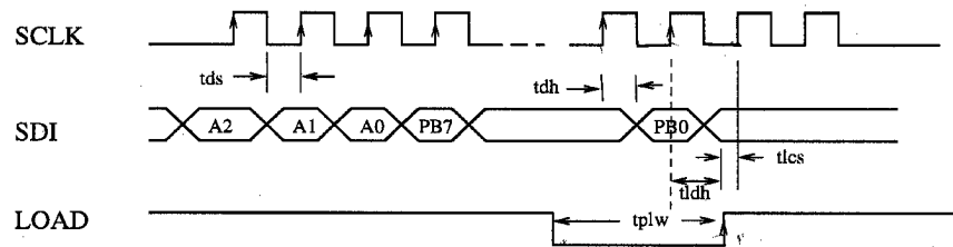
Graph 9. Write Timing
