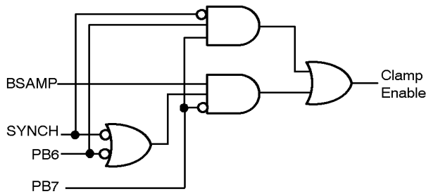
Figure 2. Clamp Enable Logic
