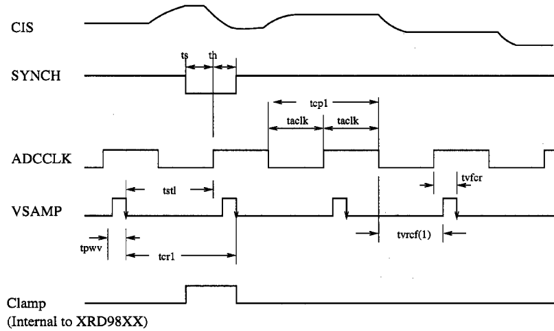
Graph 7. 1 Channel S/H Mode – Line Clamp (AC Coupled)
