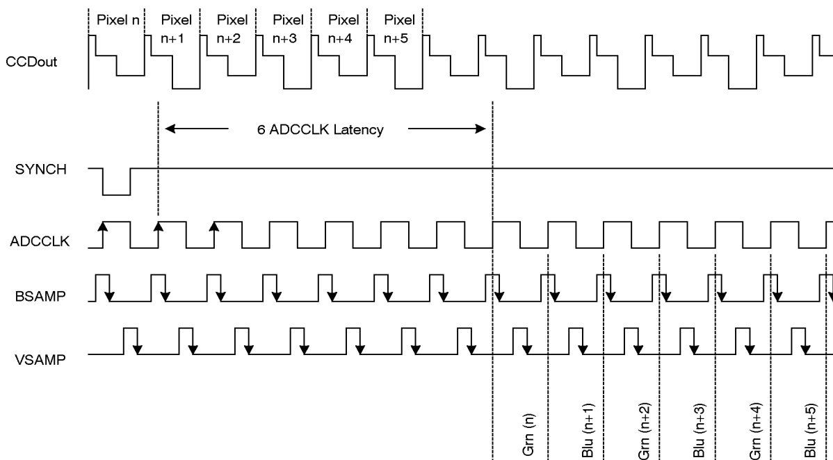
Graph 12. (B) Single Channel Bayer Mode Synchronization and ADC Timing
