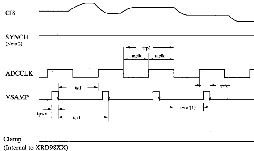
Graph 8. 1 Channel S/H Mode – No Clamp (DC Coupled)
