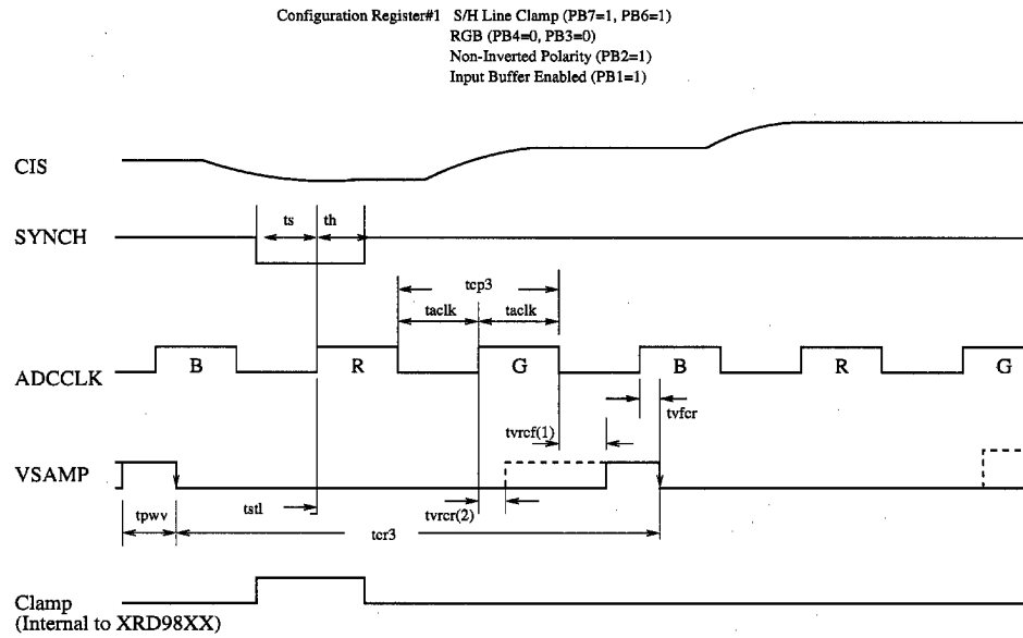
Graph 5. 3 Channel S/H Mode – Line Clamp (AC Coupled)
