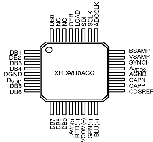
32 Lead TQFP (7 x 7 x 1.4 mm)
