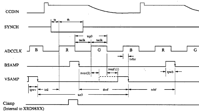
Graph 2. 3 Channel CDS Mode – Line Clamp
