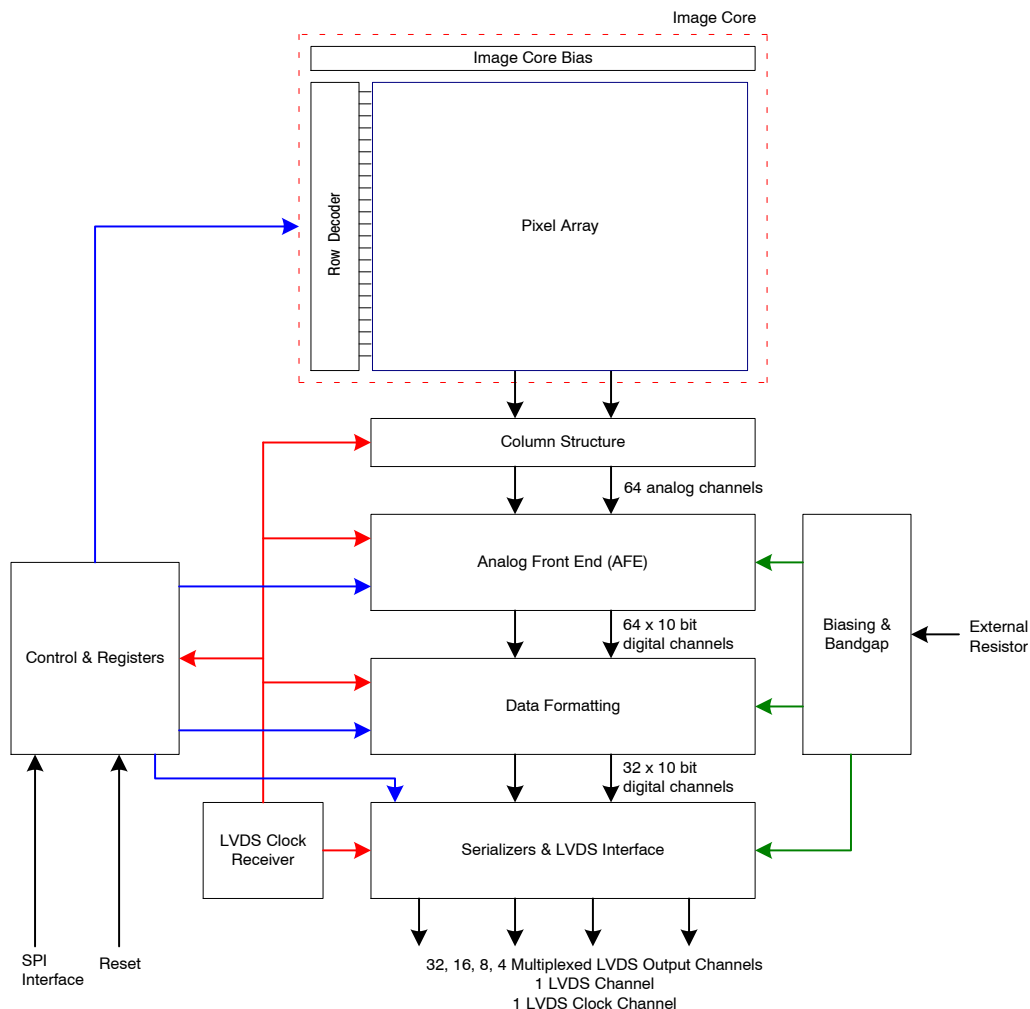
Figure 9. Block Diagram
