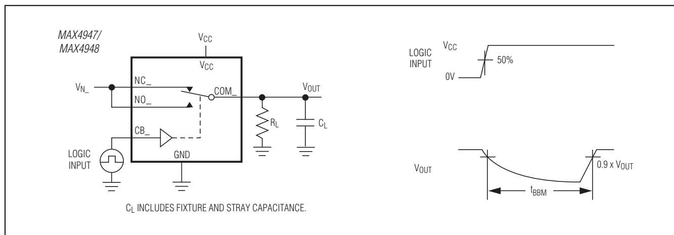
Figure 2. Break-Before-Make-Interval
