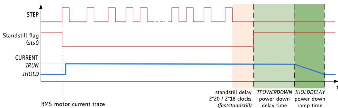
Figure 1.4 Automatic Motor Current Power Down
