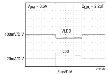
LDO Step Load Response ( 10\mu\text{A} to 10\text{mA} )
