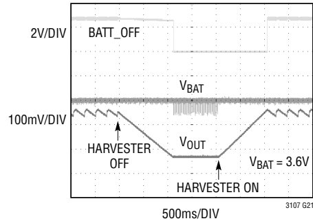
V_{OUT} Transitioning Between Harvester and Battery Power
