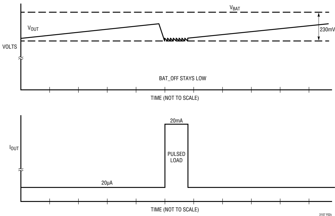
Figure 2c. V_{OUT} Waveform During a Pulsed Load When I_{HARVEST} < I_{LOAD} (Average)
