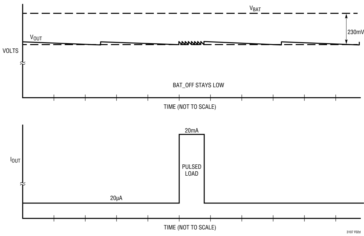
Figure 2d. V_{OUT} Waveform During a Pulsed Load When Not Harvesting
