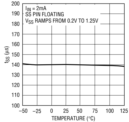
t_{\text{SS}} vs Temperature
