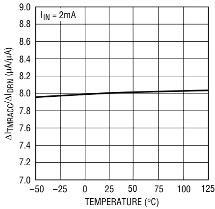
\Delta I_{\text{TMRACT}}/\Delta I_{\text{DRN}} vs Temperature
