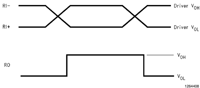
FIGURE 6. Typical Receiver Output Waveforms
