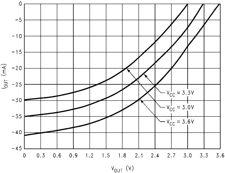
FIGURE 11. I_{OH} vs V_{OH}
