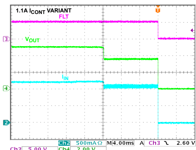
FIGURE 22. I_{LIM} WAVEFORM
