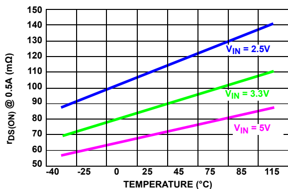
FIGURE 3. SWITCH ON-RESISTANCE AT 0.5A
