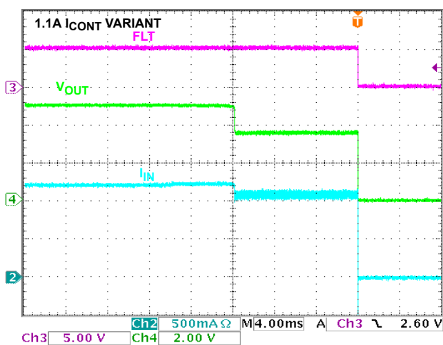
FIGURE 28. ILIM WAVEFORM
