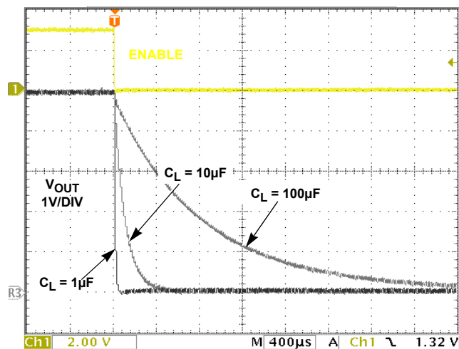
FIGURE 14. V_{OUT} TURN-OFF/FALL TIME vs C_{LOAD} . V_{IN} = 5V , R_L = 10\Omega
