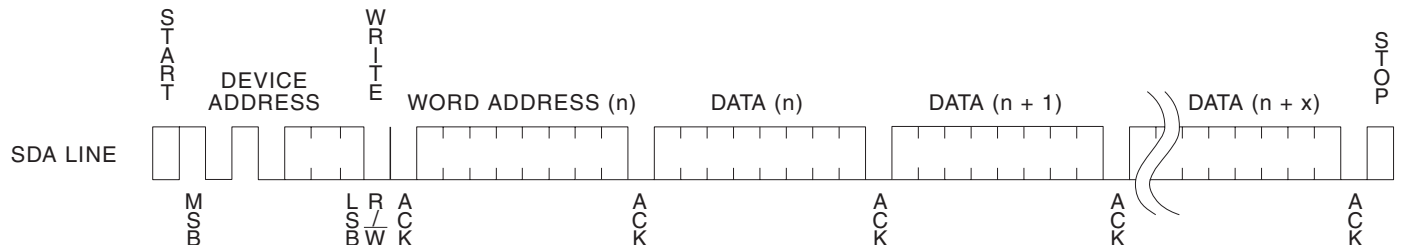
Figure 9. Page Write
