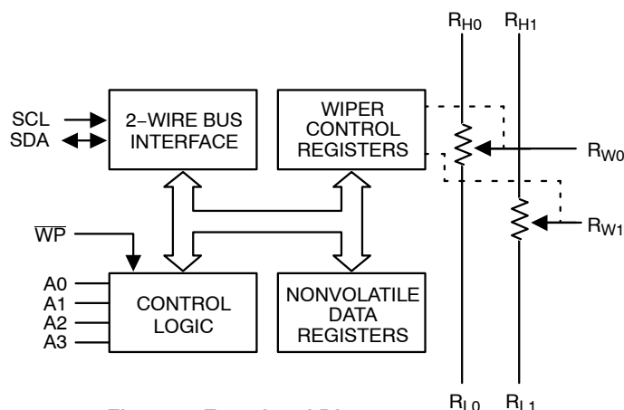
Figure 1. Functional Diagram
