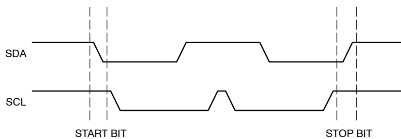
Figure 4. Start/Stop Timing
