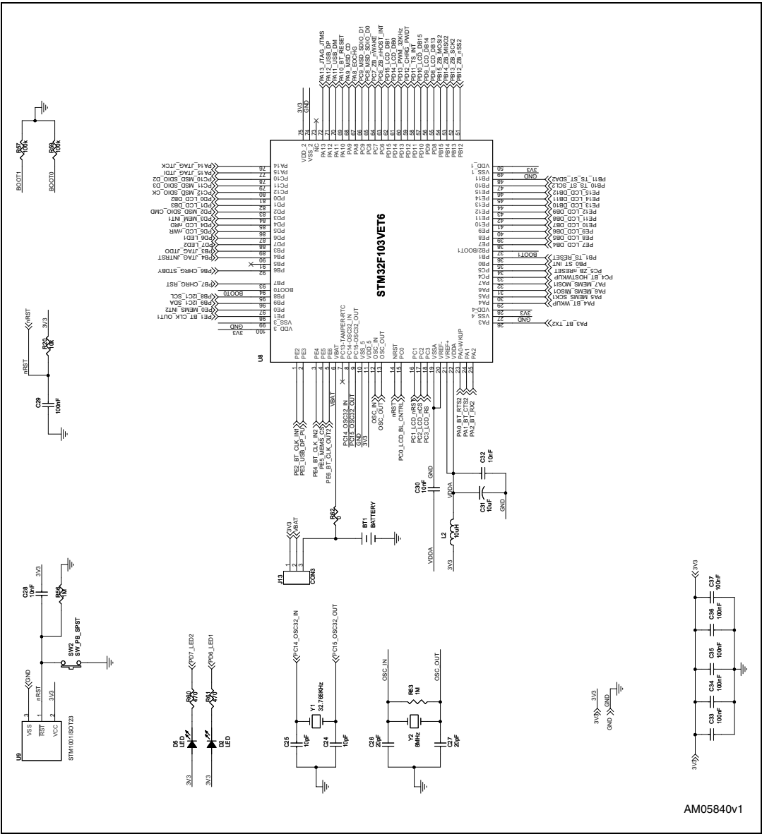
Figure 1. Microcontroller section
