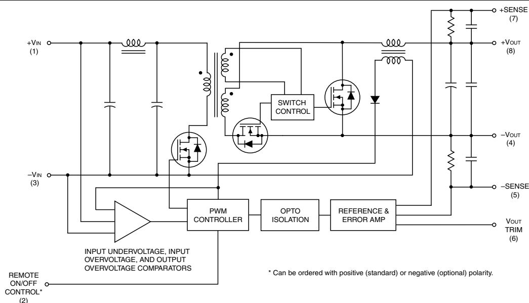
Figure 1. Simplified Schematic
