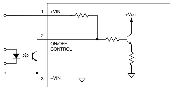
Figure 9. Driving the Negative Logic On/Off Control Pin
