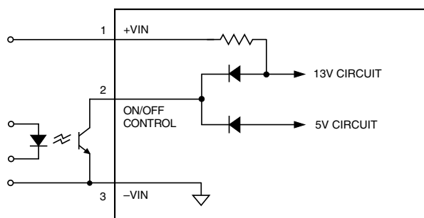
Figure 8. Driving the Positive Logic On/Off Control Pin
