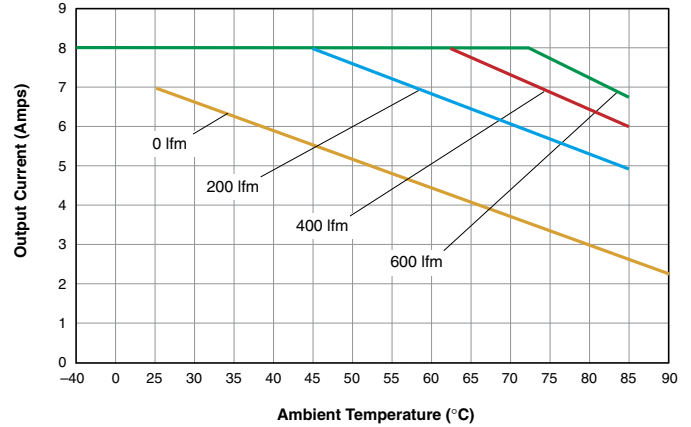
ULQ-12/8-D24 Maximum Output Current vs. Ambient Temperature ( V_{IN} = 24V , transverse air flow direction from -Output to +Output pin)
