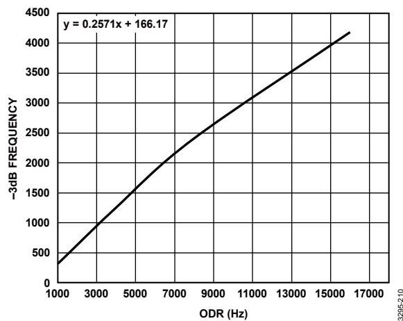
Figure 110. -3 dB Correction Factor, HR Mode
