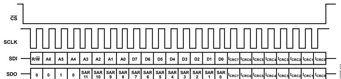
Figure 103. SAR ADC/Diagnostic Mode—CRC Enabled
