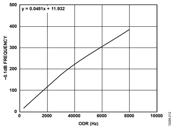
Figure 111. -0.1 dB Correction Factor, LP Mode
