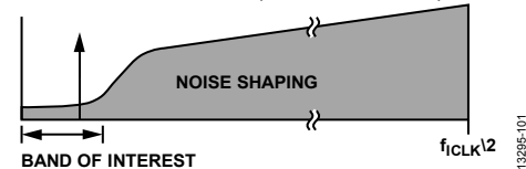
Figure 83. \Sigma - \Delta ADC Operation, Majority of Noise Energy Shifted Out of the Band of Interest (Linear Scale X-Axis)
