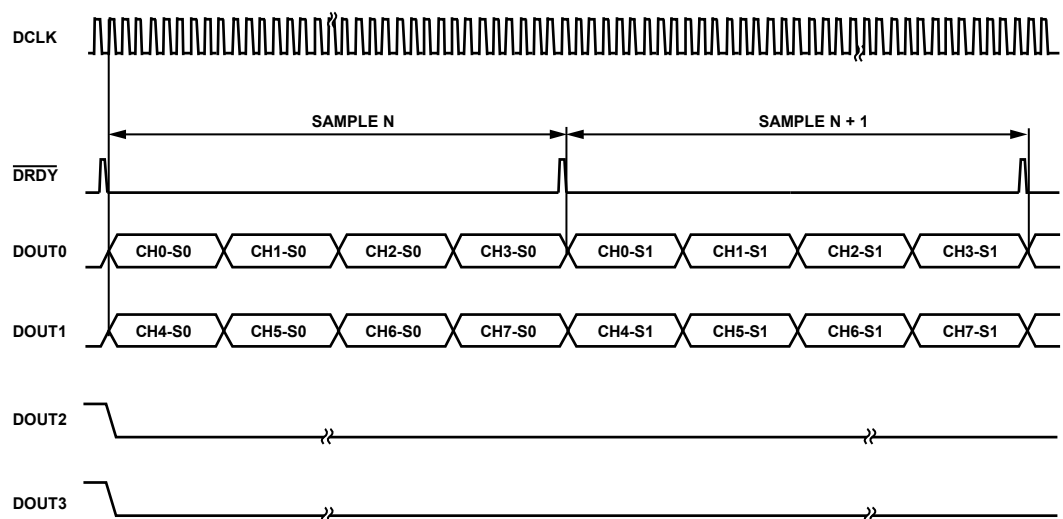
Figure 117. FORMAT0 = 0 , FORMAT1 = 1 —Channel 0 to Channel 3 Share DOUT0, and Channel 4 to Channel 7 Share DOUT1 (S0 Means Sample 0 and S1 Means Sample 1)
