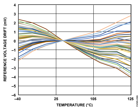
Figure 54. Internal Reference Voltage Drift
