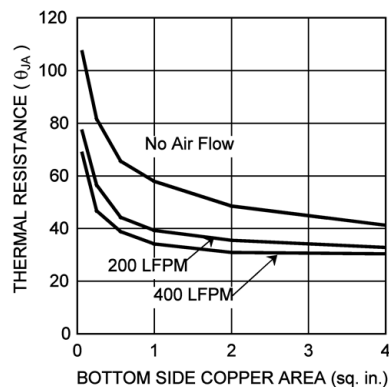
Figure 42. Thermal Resistance vs PCB Area
