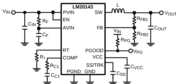
Figure 32. Typical Application Circuit
