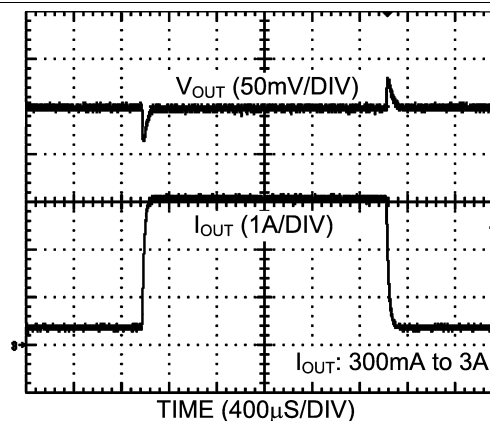
Figure 22. Load Transient Response
