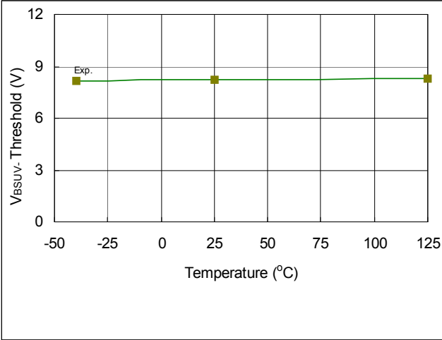
Fig. 35 V_{BSUV-} Threshold vs. Temperature
