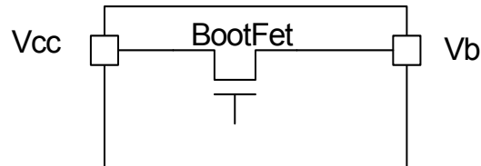
Figure 8: Semplified BootFET connection
