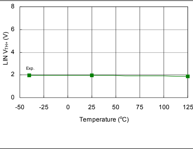
Fig. 39. LIN V_{TH+} vs. Temperature
