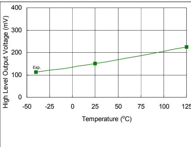
Fig. 37. High Level Output Voltage vs. Temperature
