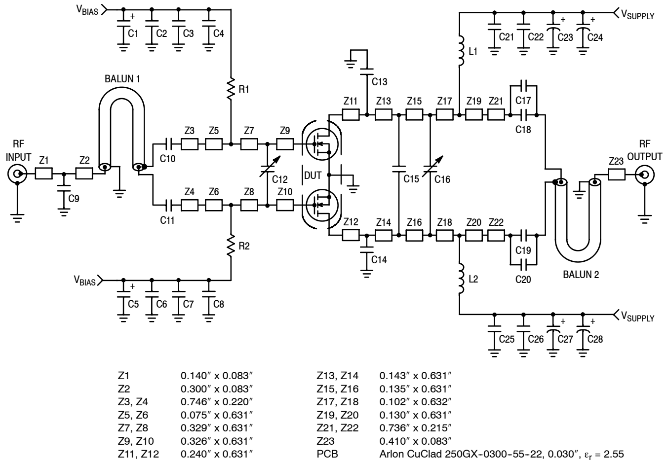
Figure 2. MRF6VP121KHR6(HSR6) Test Circuit Schematic
