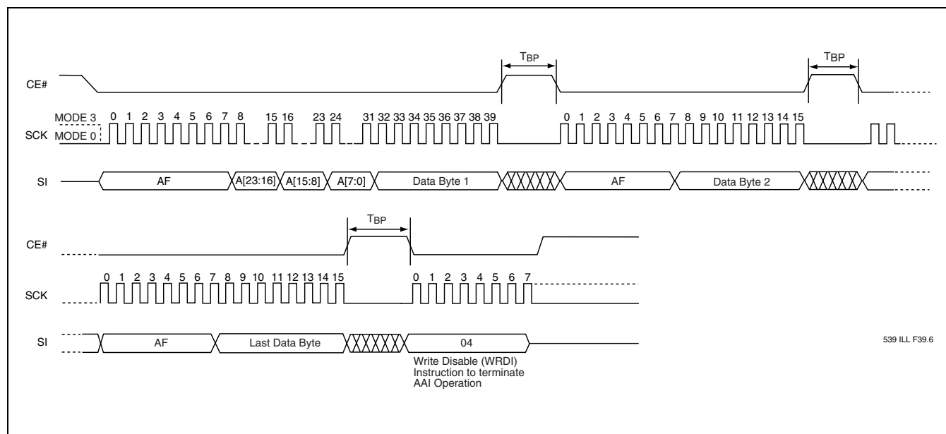
FIGURE 6: AUTO ADDRESS INCREMENT (AAI) PROGRAM SEQUENCE
