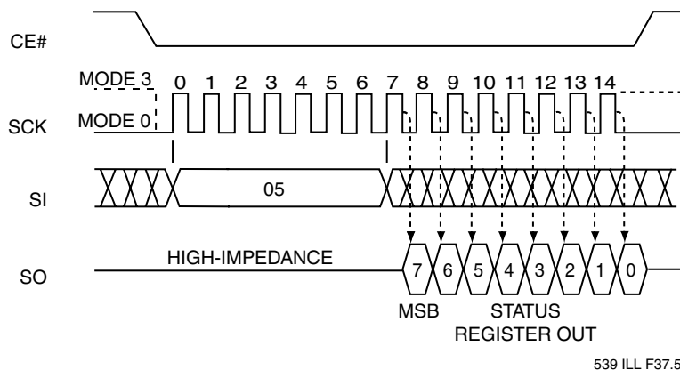
FIGURE 10: READ-STATUS-REGISTER (RDSR) SEQUENCE
