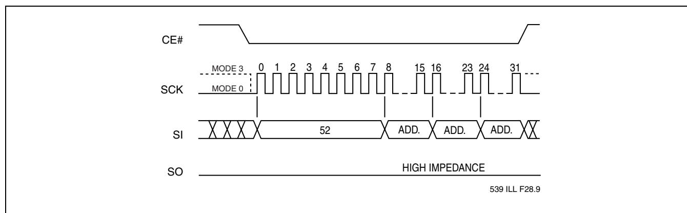
FIGURE 8: BLOCK-ERASE SEQUENCE
