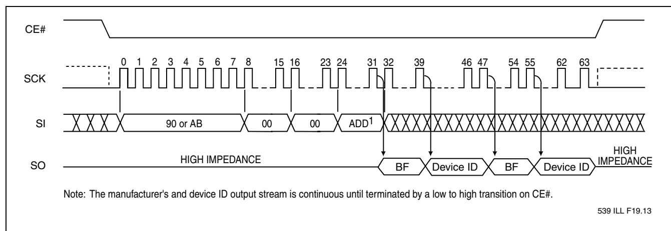
FIGURE 14: READ-ID SEQUENCE
